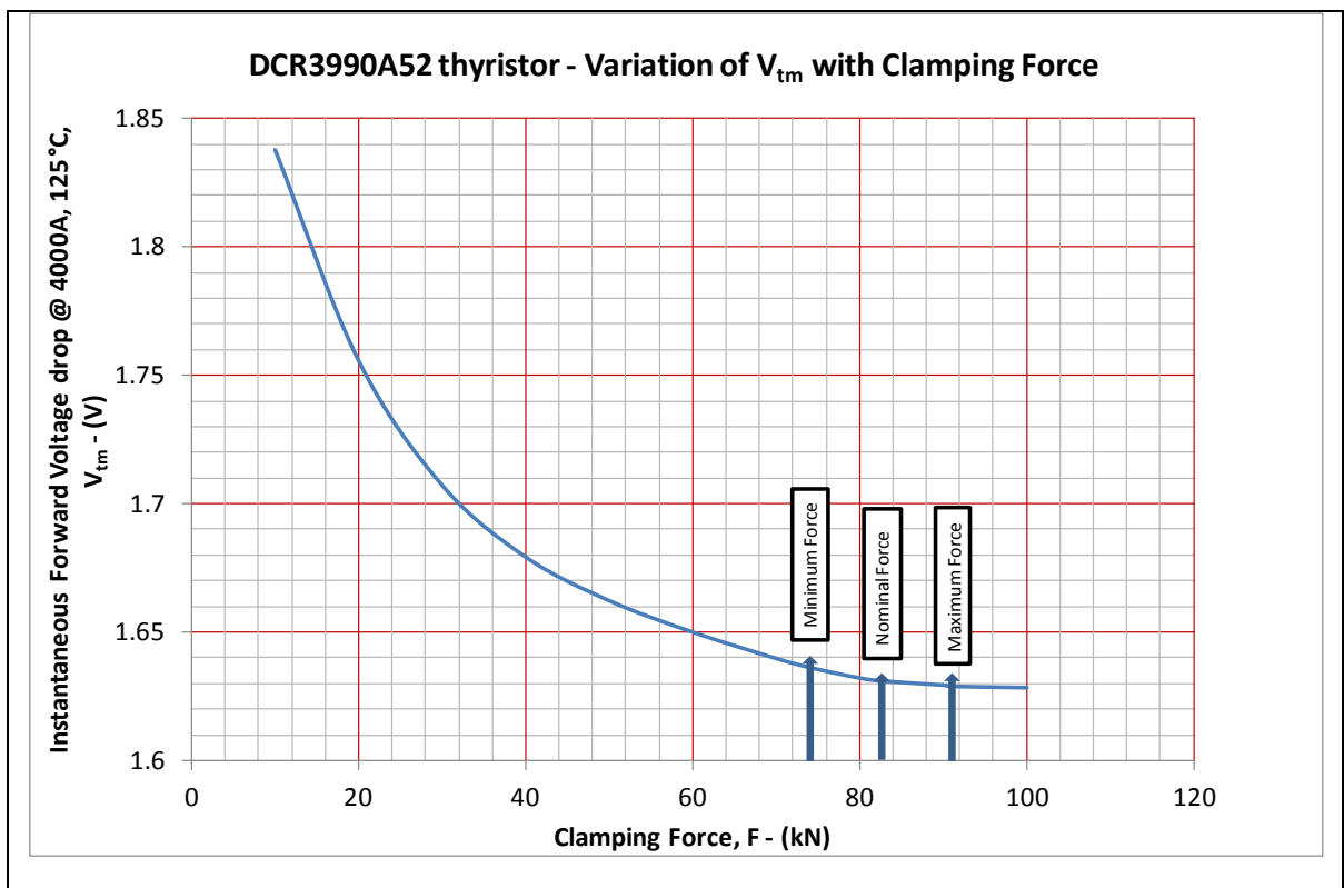
Figure 3 DCR3990A52 thyristor – variation of Forward Voltage Drop with clamping
