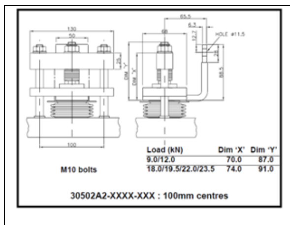
Figure 6 Typical Clamp for Single Side Cooling
