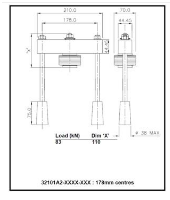
Figure 5 Typical Clamp for Double Side Cooling
