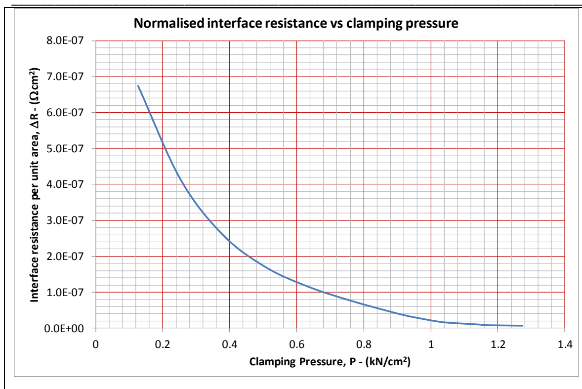
Figure 4 Normalised interface resistance variation with clamping pressure
