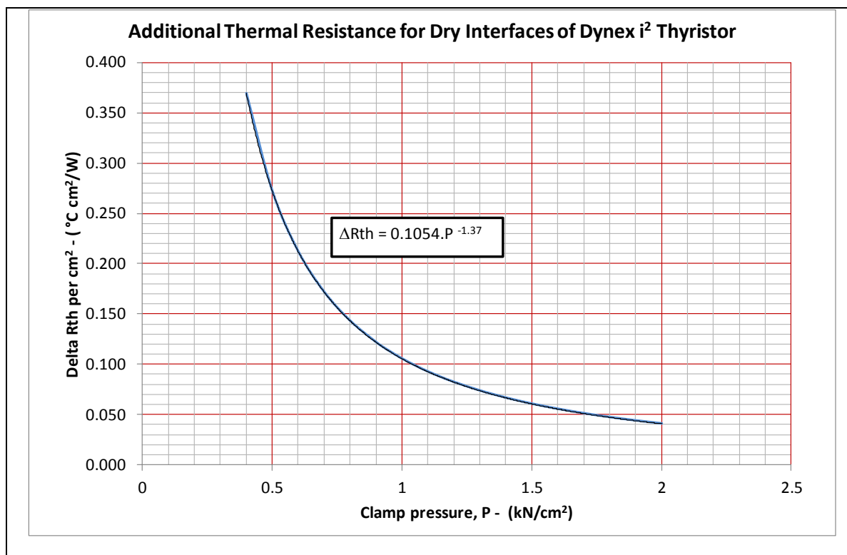
Figure 1 Thermal resistance of dry interfaces of a fully floating thyristor.
