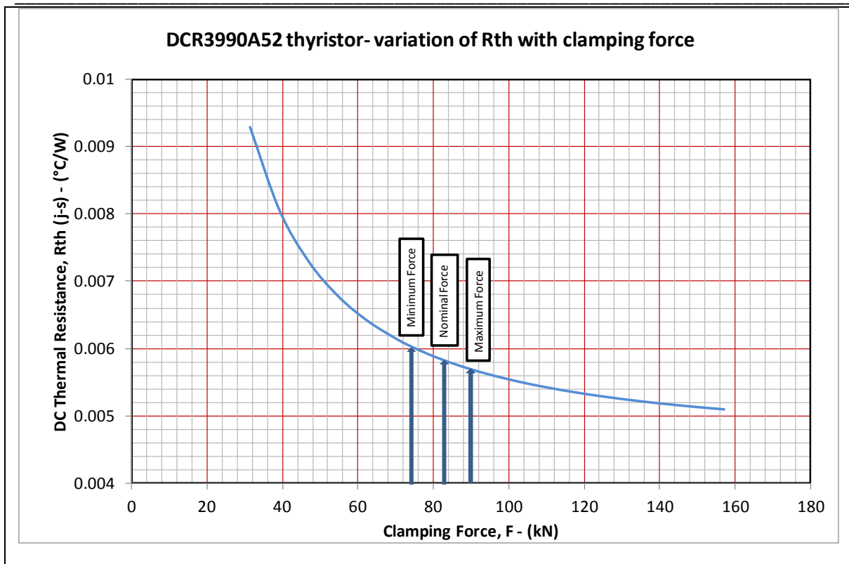
Figure 2 DCR3990A52 thyristor – variation of thermal resistance with clamping force.
