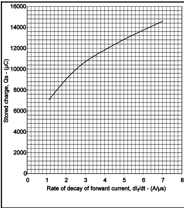
Fig.4 Stored charge
