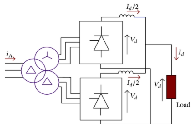
Figure 2. A 12 pulse bridge rectifier consisting of two phase shifted 6 pulse bridges with connected outputs
