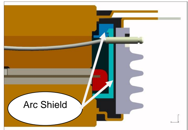
Fig 6. Schematic diagram of arc shield design
