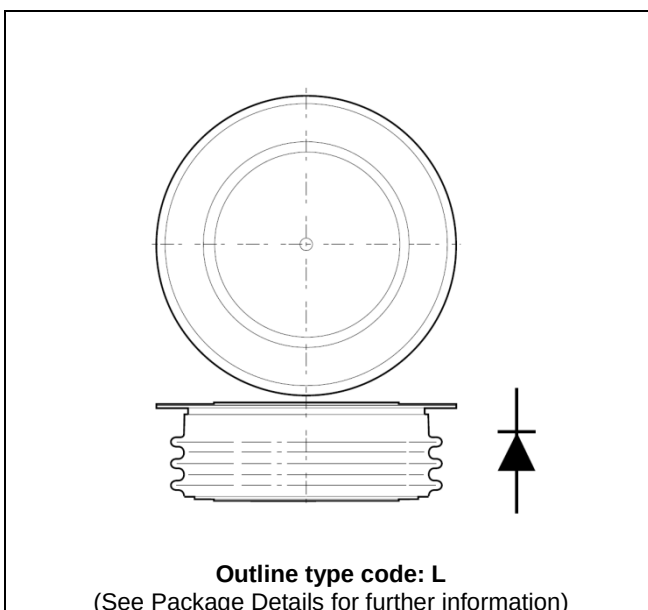
Fig. 1 Package outline
