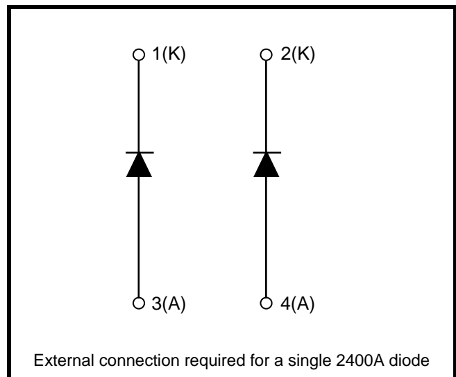
Fig. 1 Circuit configuration
