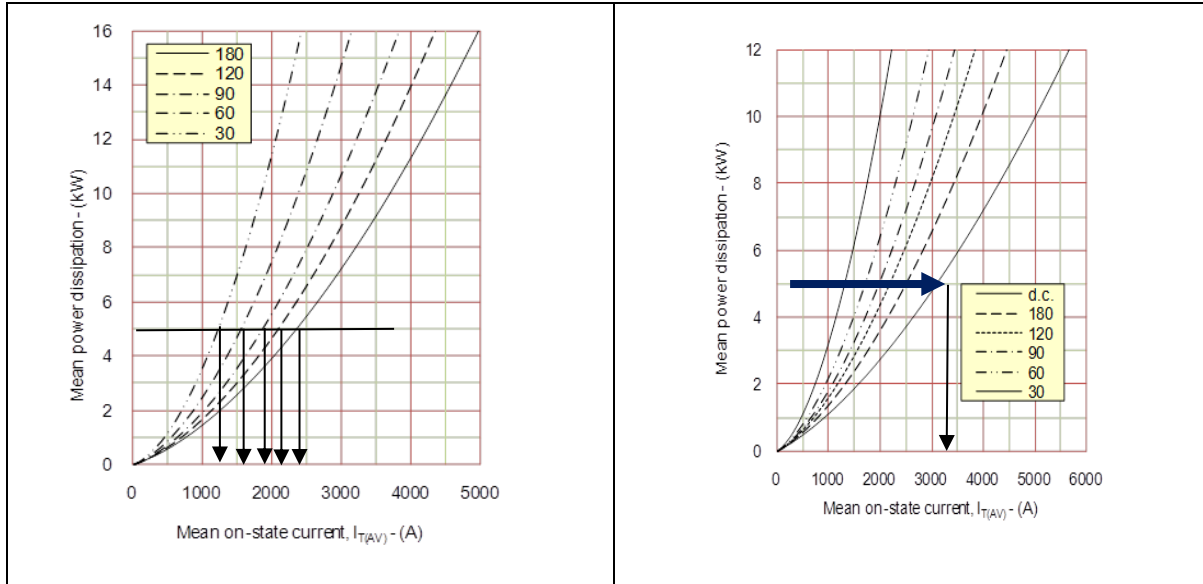
Fig.3 On-state power dissipation – sine wave
