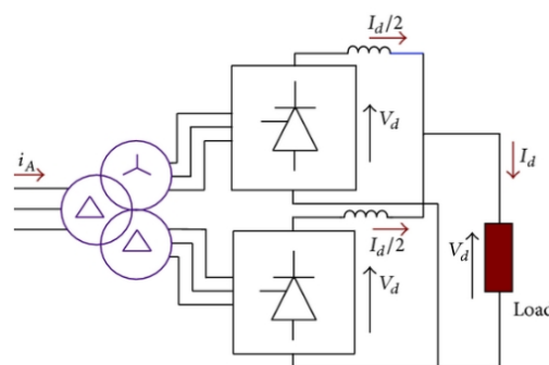
Figure 2. A 12-pulse bridge rectifier consisting of two phase shifted 6 pulse bridges with connected outputs
