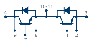
Half Bridge - M1HM
