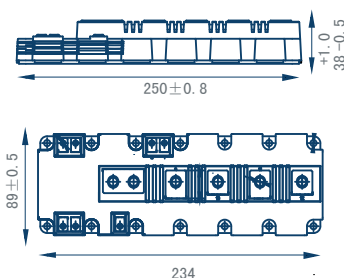
Package Type: H1
