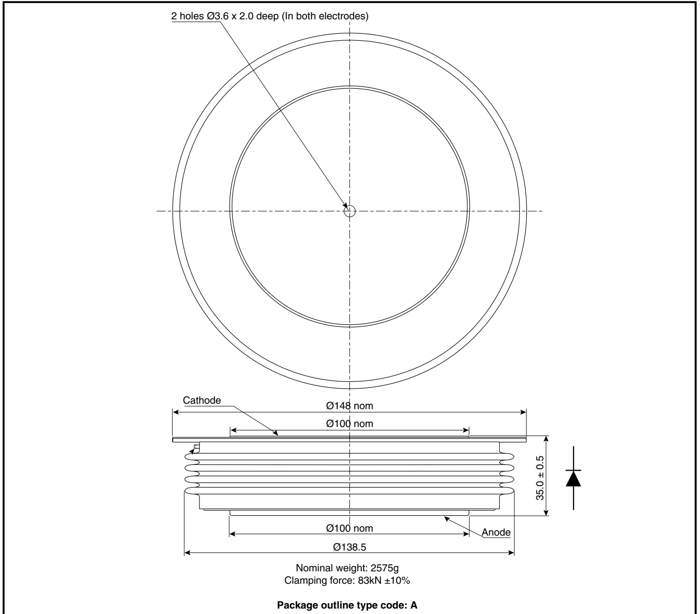
Fig. 8 Package details
