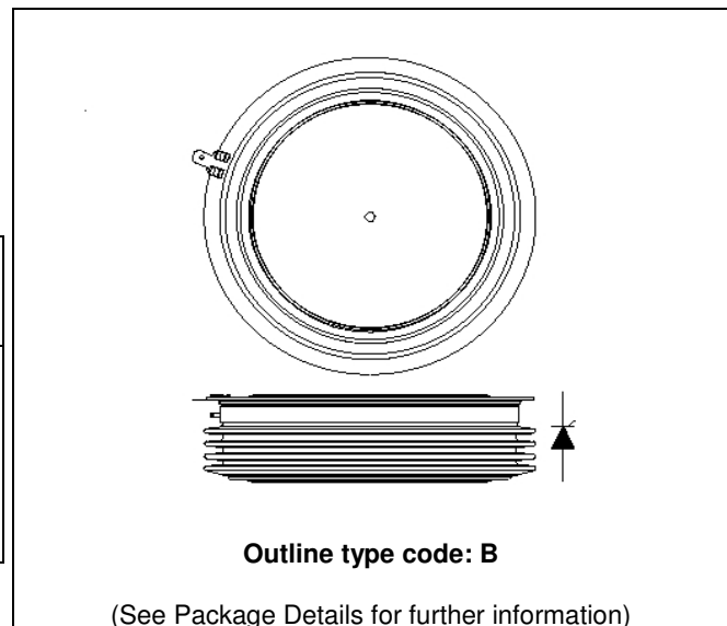
Fig. 1 Package outline
