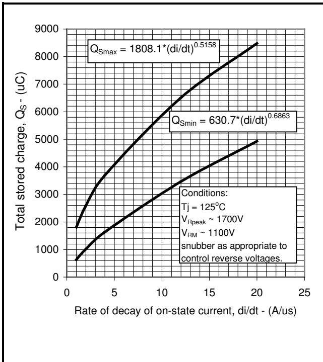
Fig. 12 Stored Charge
