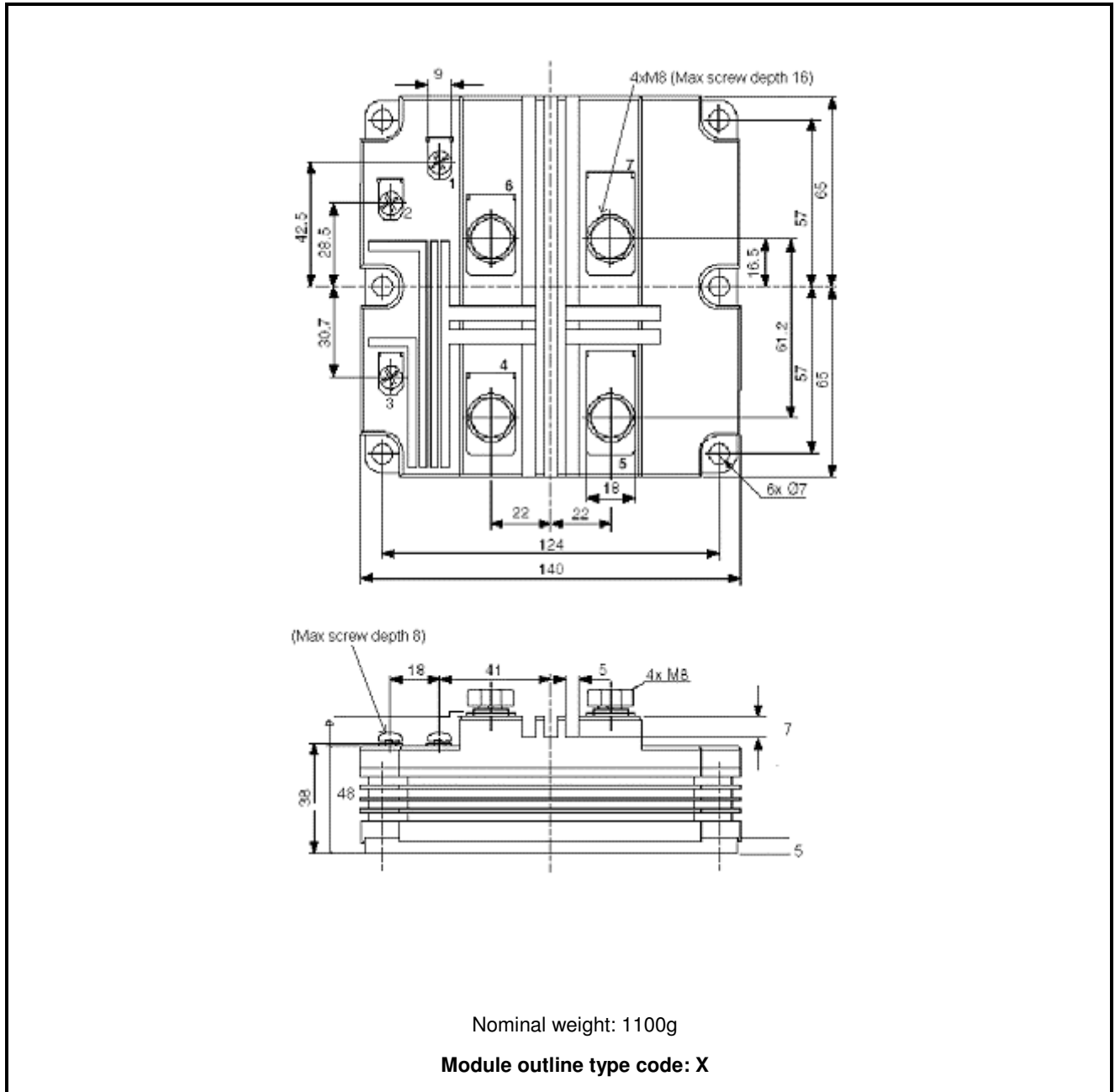
Fig. 11 Outline drawing
