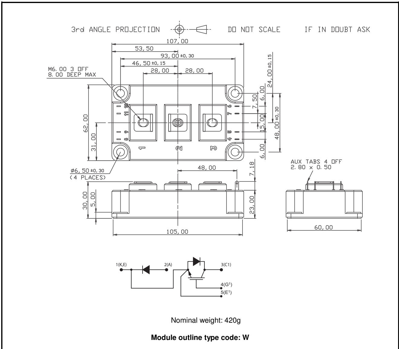
Fig.11 Package details
