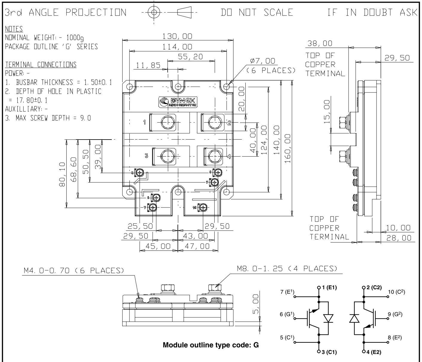
Fig.11 Package details
