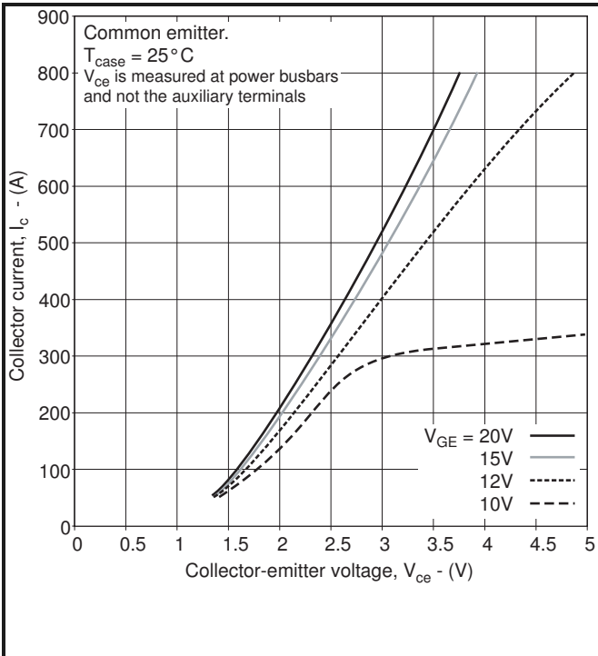
Fig.3 Typical output characteristics @ 25°C
