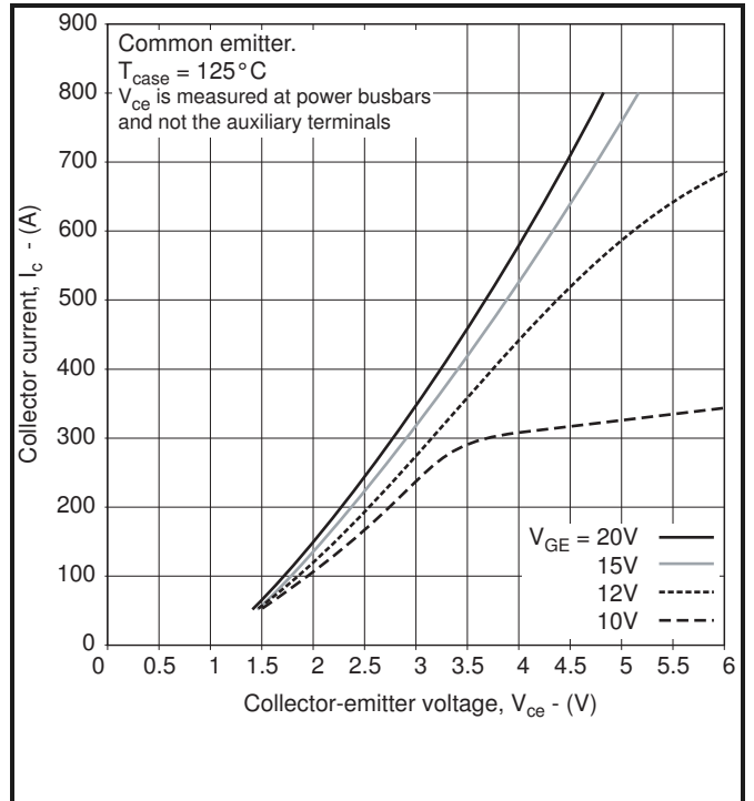
Fig.4 Typical output characteristics @ 125°C
