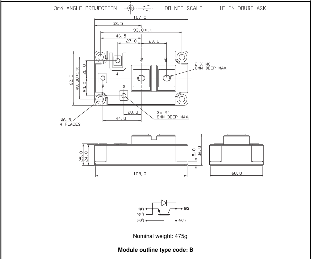
Fig.11 Package details
