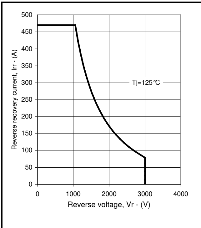
Fig.7 Diode reverse bias safe operating area
