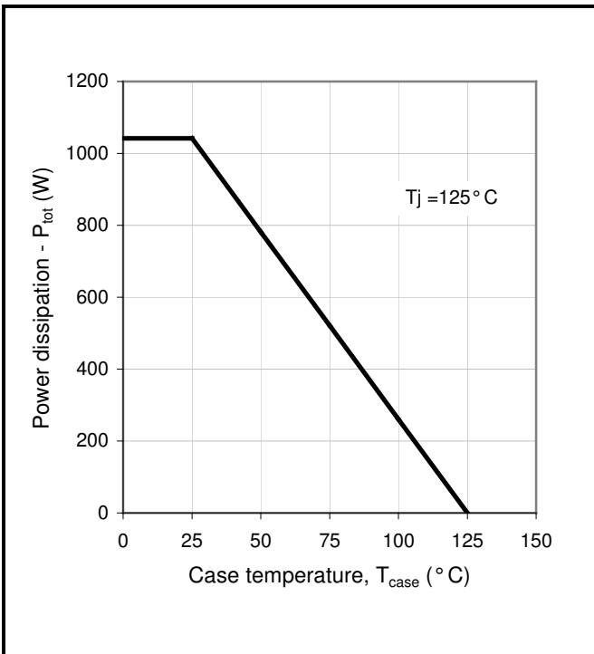
Fig.5 Power dissipation
