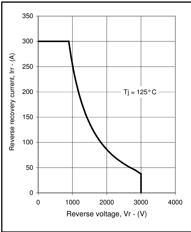
Fig.7 Diode reverse bias safe operating area
