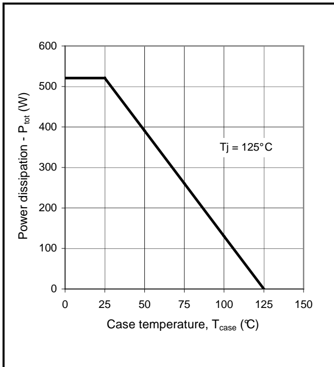
Fig.5 Power dissipation
