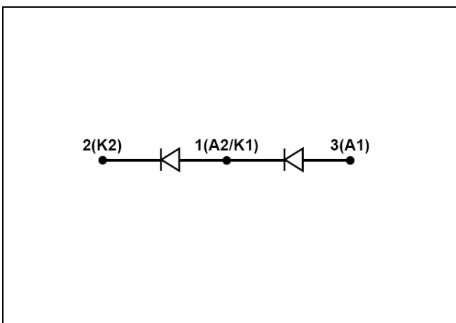
Fig. 1 Circuit diagram
