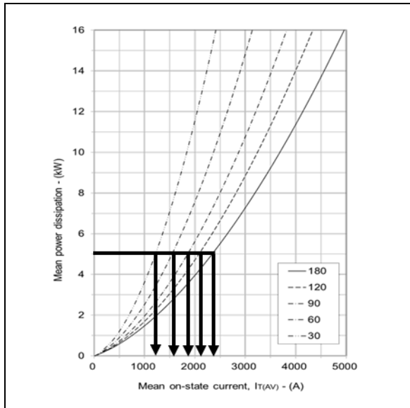
Fig.3 On-state power dissipation – sine wave
